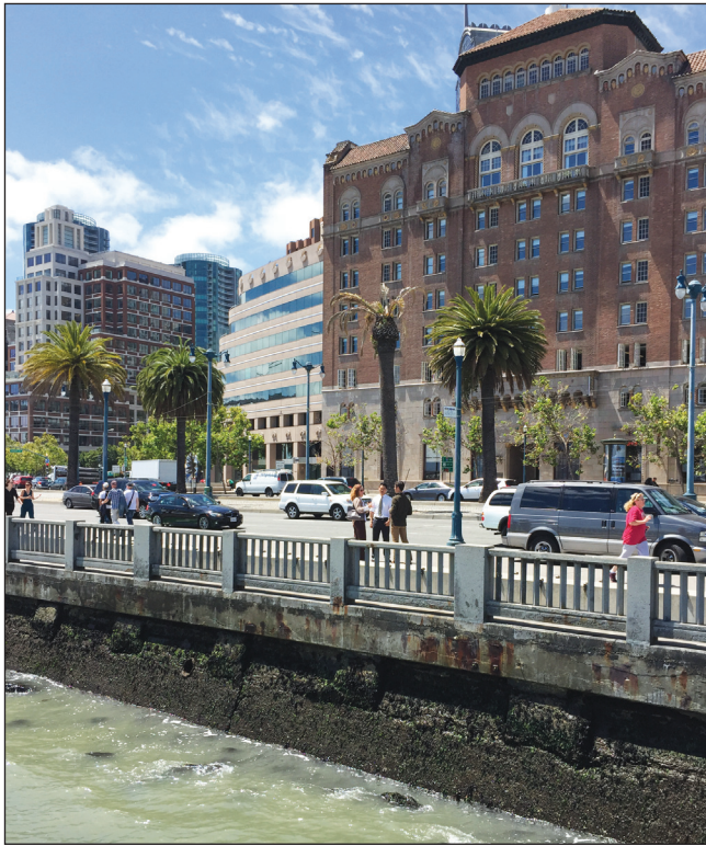
Figure 1. Seawall in San Francisco, California. Seawalls are fixed walls made of reinforced concrete or steel, often combined with wooden pilings treated with creosote. They are designed to retain unconsolidated fill on the landward side, which contains the footings of buildings and other infrastructure. Relieving platforms constructed of wood, or concrete and steel, hold the walls in place. These walls were essential for bringing ships directly into urban quays to efficiently load and unload cargo or passengers.
