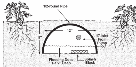
Leaching Chamber
